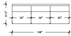
SOFA PLUS C (36" SEATS)
