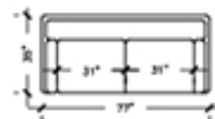
APARTMENT SOFA W: 77" D: 35" H: 33" ARM H: 30" SEAT D: 24"
